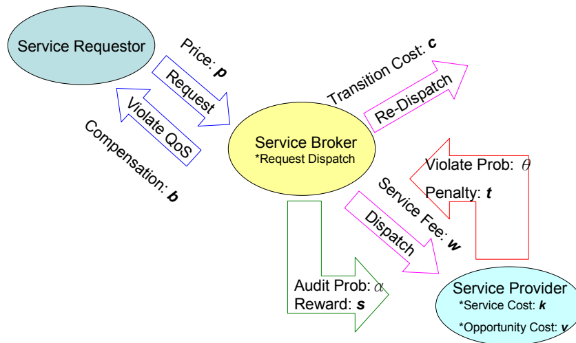
Figure 3: Service Architecture and Contract Rules
