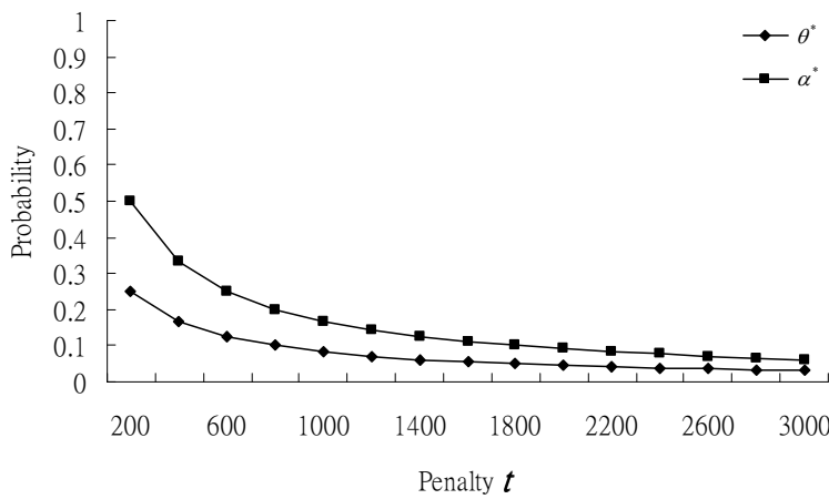
Figure 6: Fixed Reward with Increased Penalty
