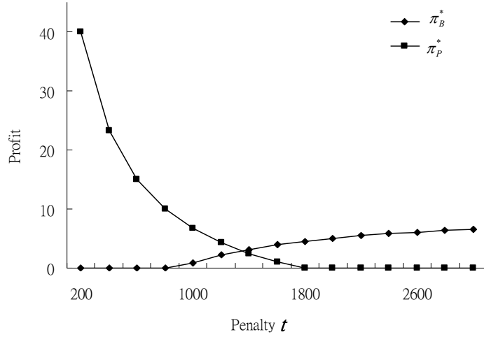
Figure 8: Expected Equilibrium Profit against Increased Penalty
