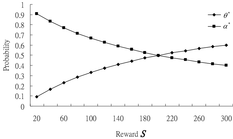
Figure 5: Fixed Penalty with Increased Reward
