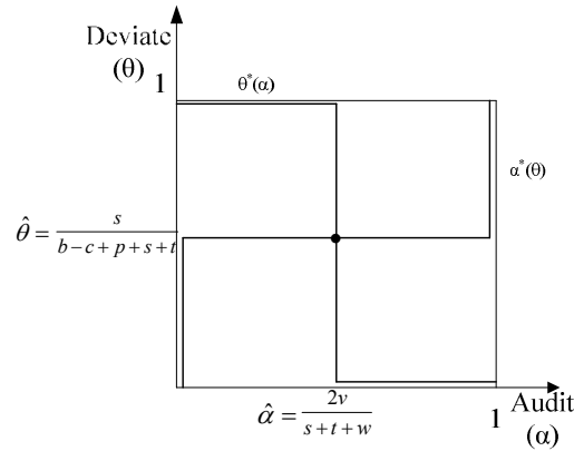
Figure 4: Best Response Function for Broker and Provider
