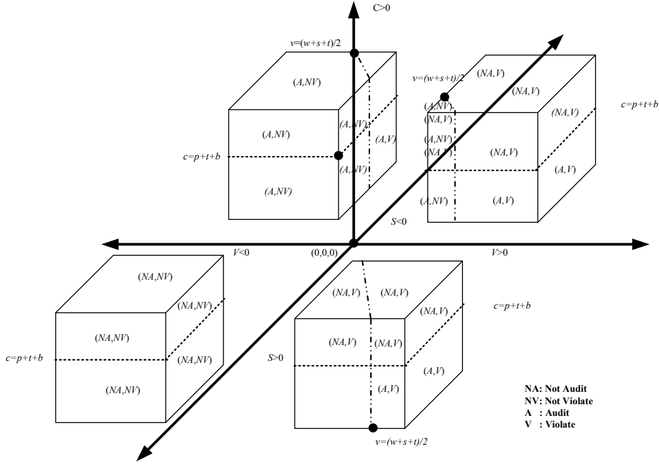
Figure 9: Pure Strategy Nash Equilibrium
