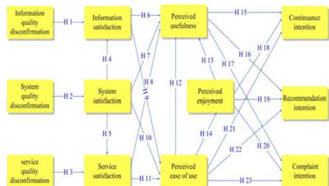
Fig. 1. Research model
